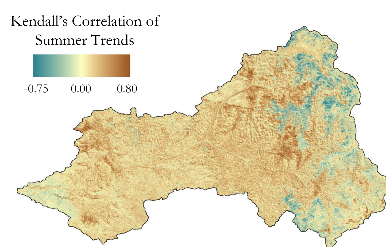
Figure 2. Kendall's Correlation conducted on detrended Normalized Difference Snow and Ice Index values from 2000 - 2016. Areas of drastic negative and positive trends lay within the zones of accumulation and ablation of perennial glaciers.
