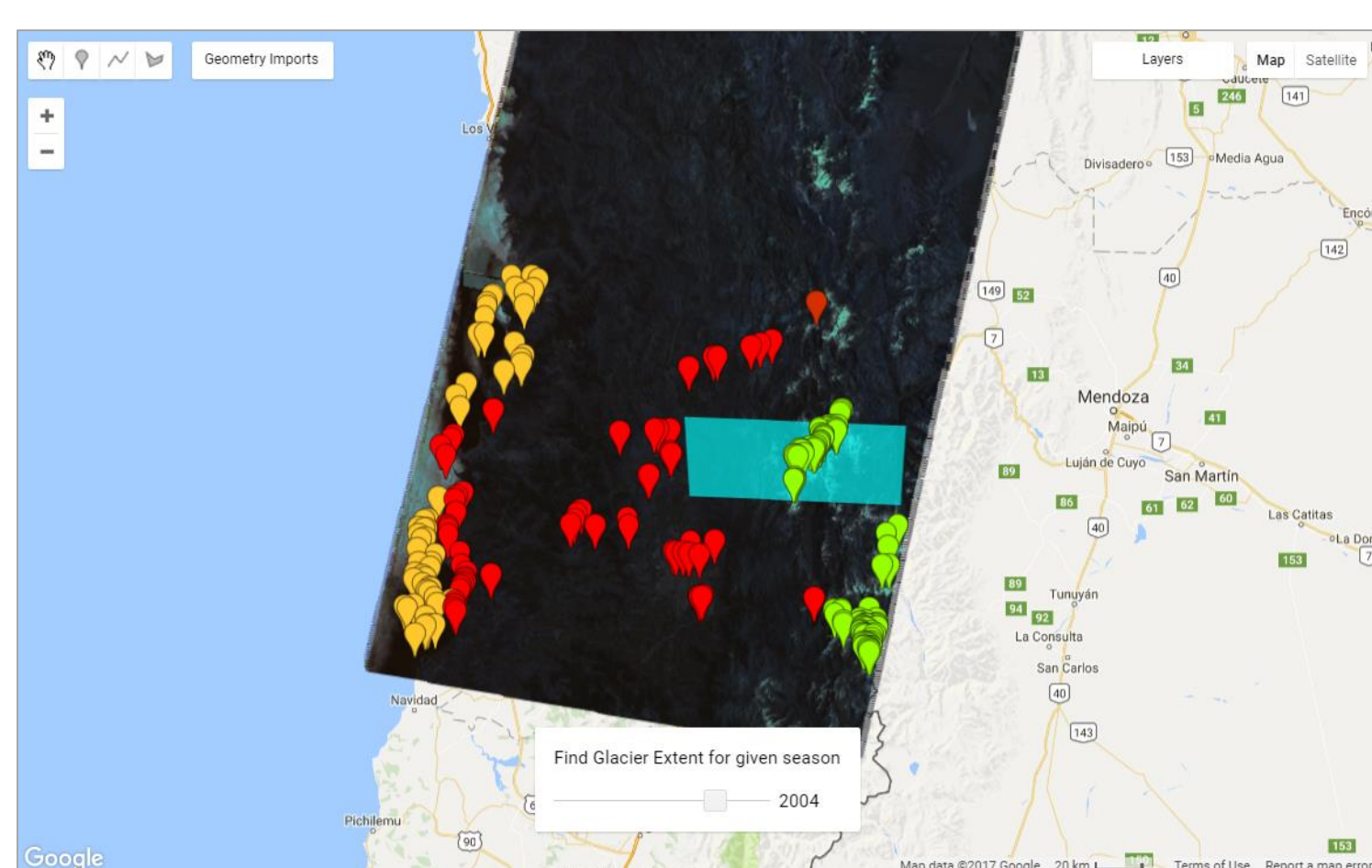
Figure 1. Supervised hard classification of glaciated area in 2004. Spectral signatures from Landsat imagery are used to differentiate ice from non-ice. The classification and area of glacial can be applied to any year of Landsat coverage. The glaciated area within the blue bounding box is 376.95 km 2 .
