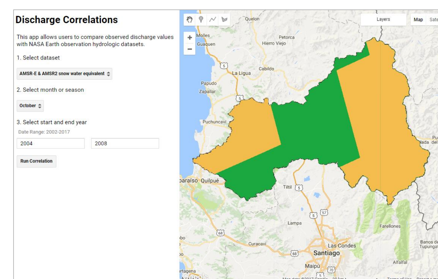
Figure 3. Preview of Pearson's Product-moment correlation coefficient tool relating in situ river discharge measurements (dependent) and important hydrologic indicator environmental variables derived from NASA sensors (independent).
